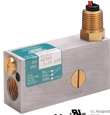
Shown with optional 1/2" conduit connector.
